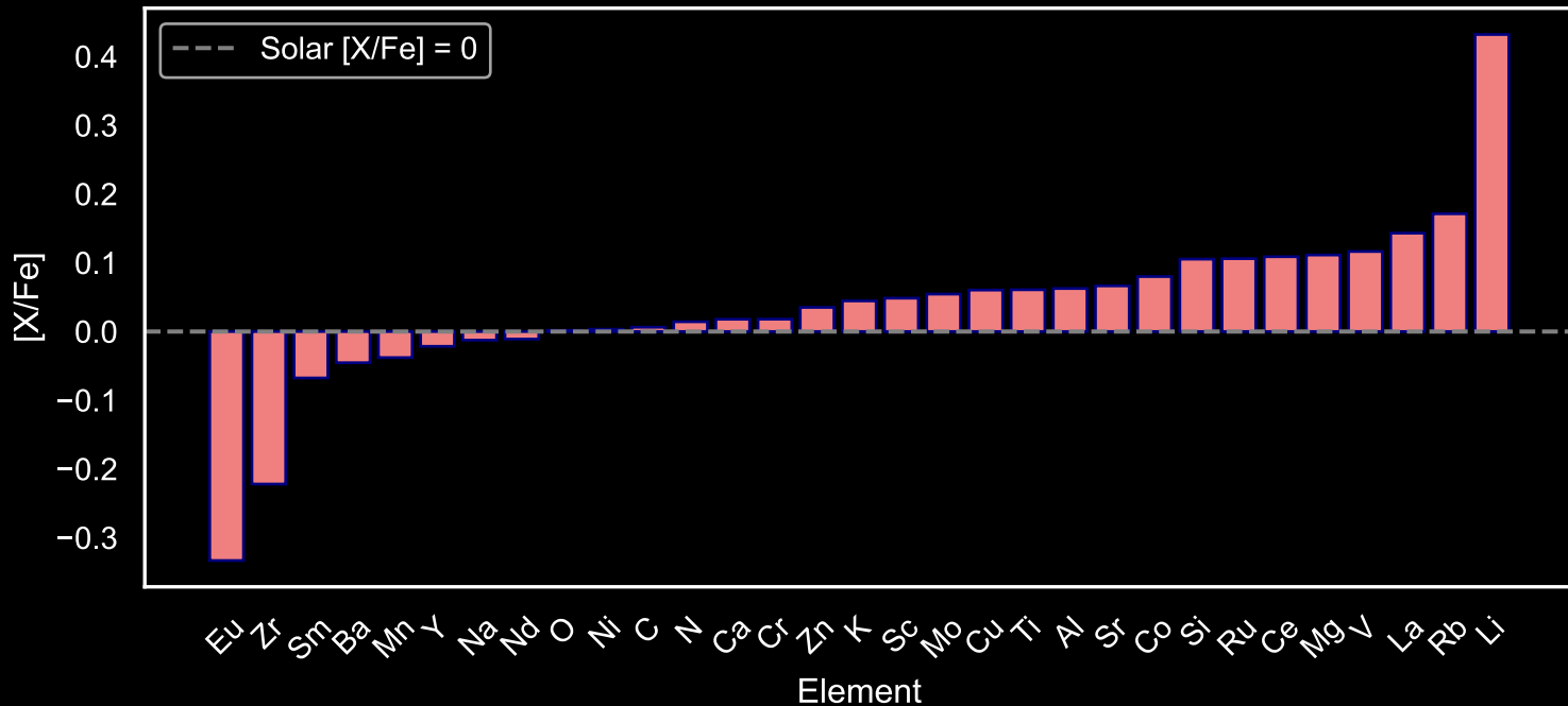
Abundance Pattern for GALAH Main Sequence Stars: Star Field [82] (N=109)
