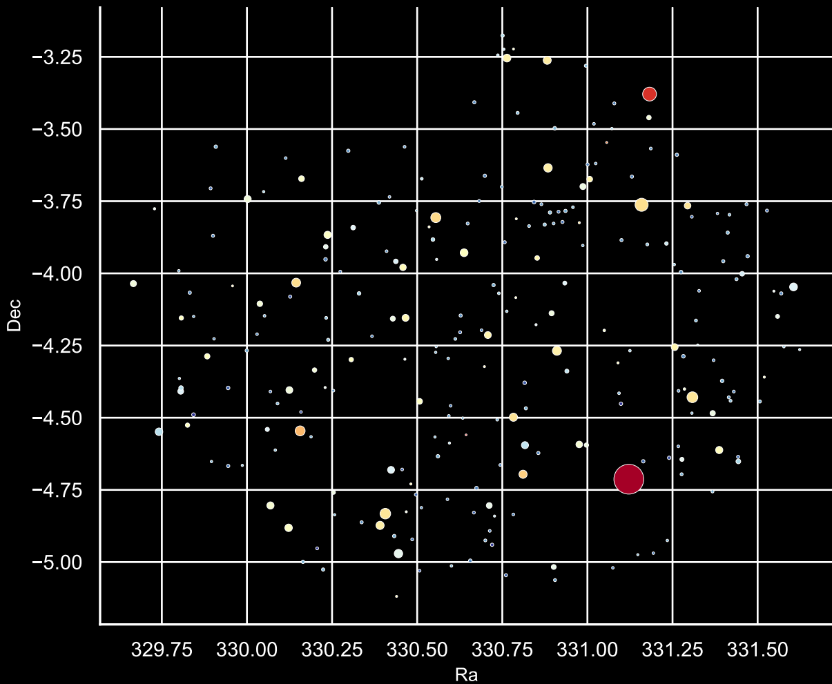
Field [82] Ra [330.71] Dec [-4.22] Stars: 244
