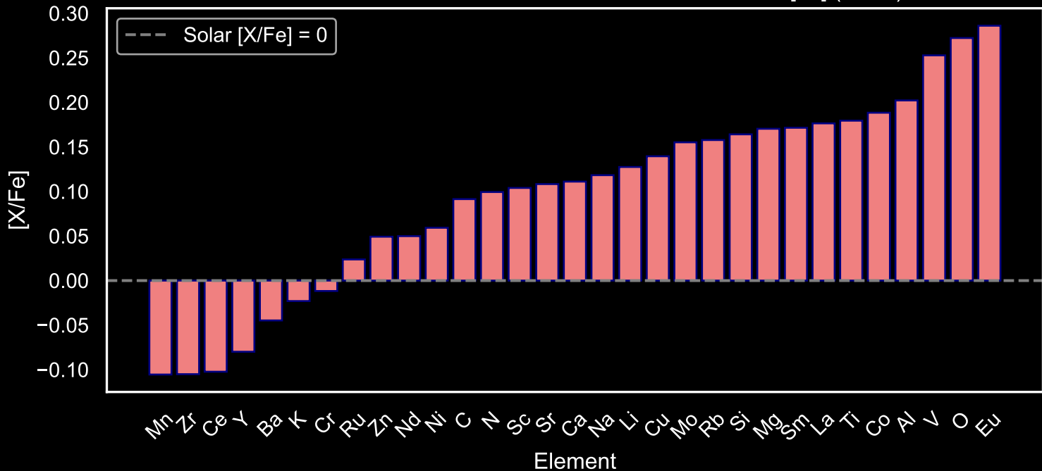
Abundance Pattern for GALAH Red Giants: Star Field [82] (N=62)
