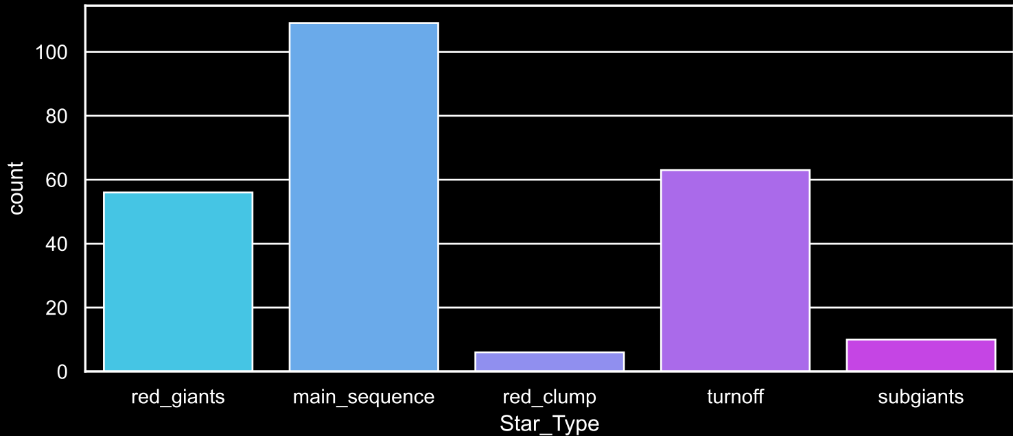
Field [82] Count plot of Star Type
