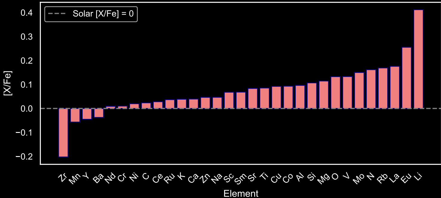
Abundance Pattern for GALAH Star Field [82] (N=244)
